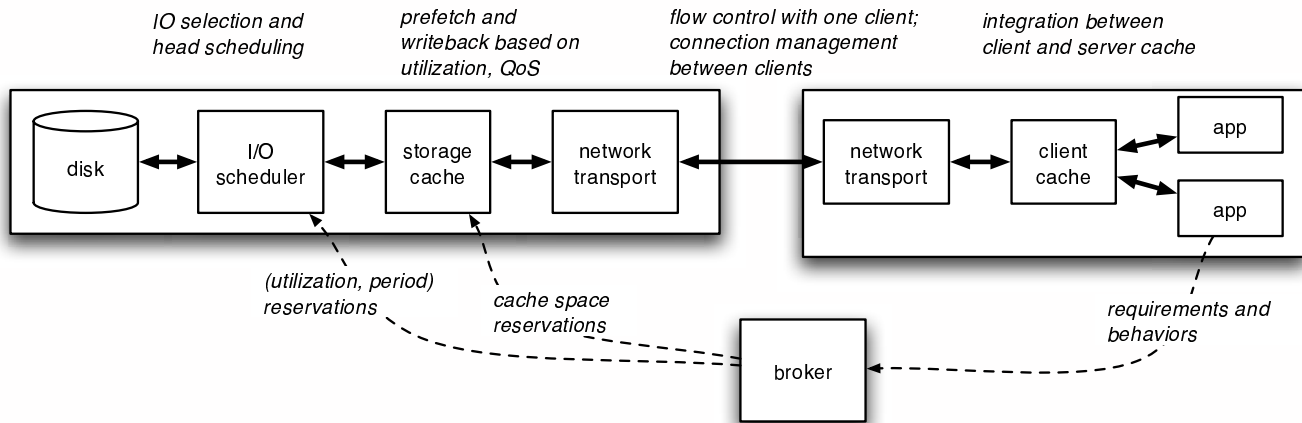
Figure 1. The stages in the data pipeline.
