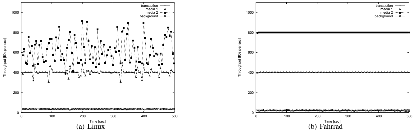
Figure 3. Behavior of mixed workload during 500 seconds, with and without Fahrrad. Points are the average for 5-second intervals.
