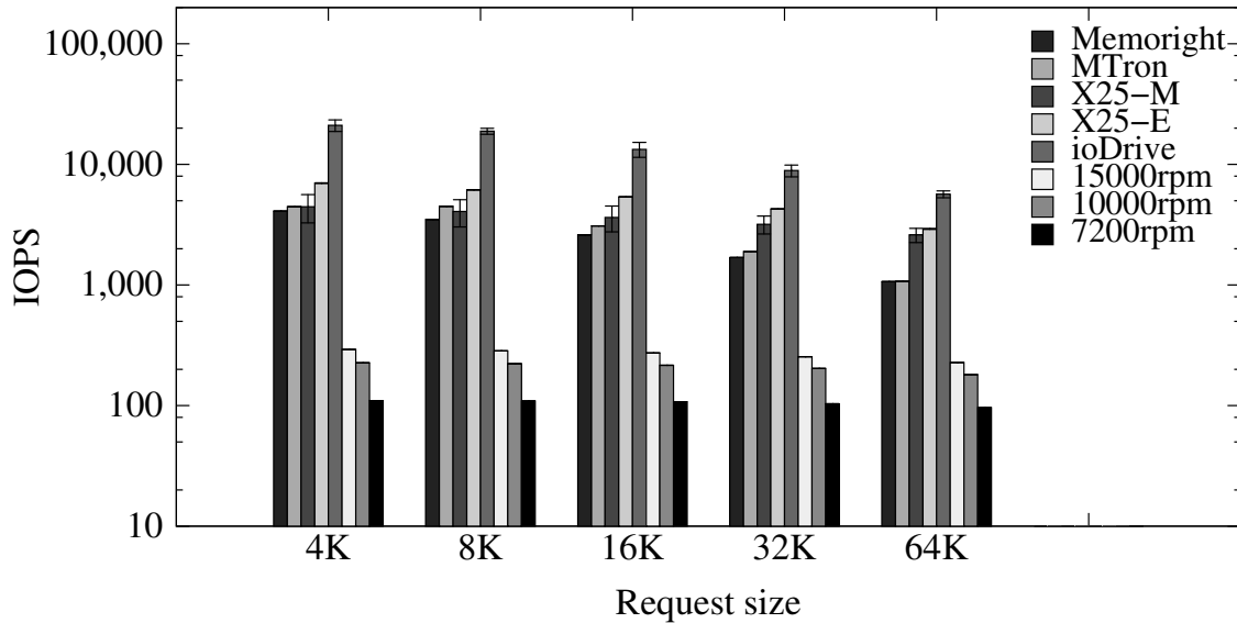
Fig. 3. Random reads
