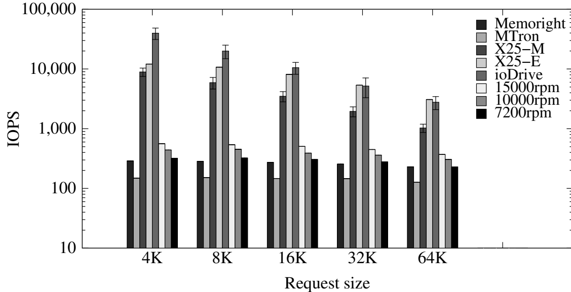
Fig. 4. Random writes
