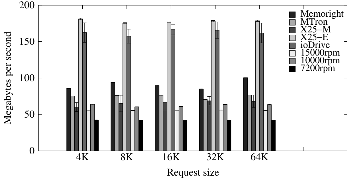
Fig. 2. Sequential writes
